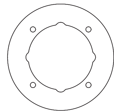
Lawn Mower Engine Sealed Grommet
